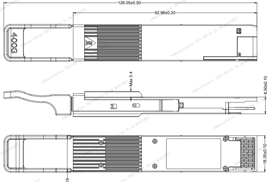
Figure 7.1 Package Dimensions
