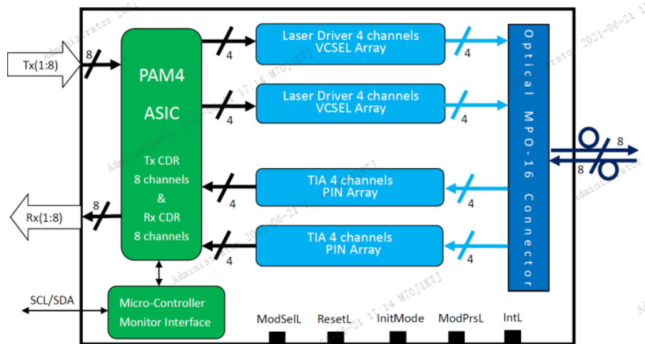
Figure 2.1 Transceiver Block Diagram
